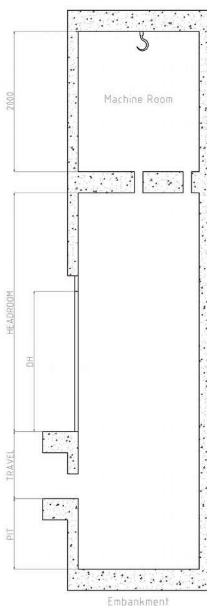
Vertical section
