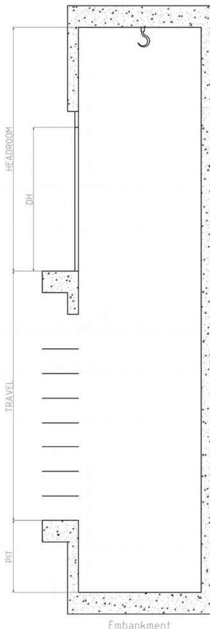
Vertical section
