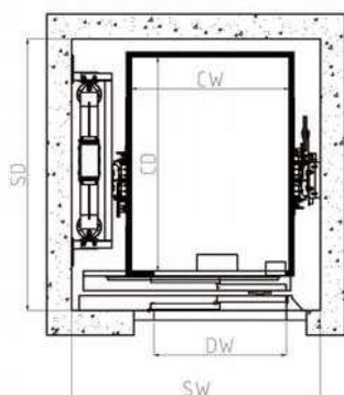
FTT - Opposite guide rail - 2:1
