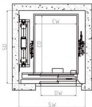
MRS - Opposite guide rail - 2:1
